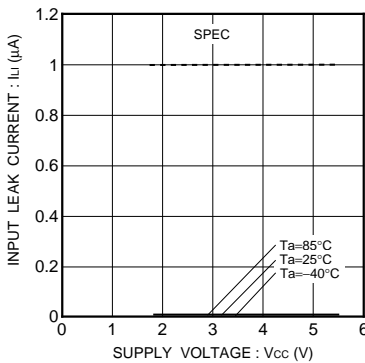
Fig.21 Input leakage current I_{IL} (A0,A1,A2,SCL,WP)
